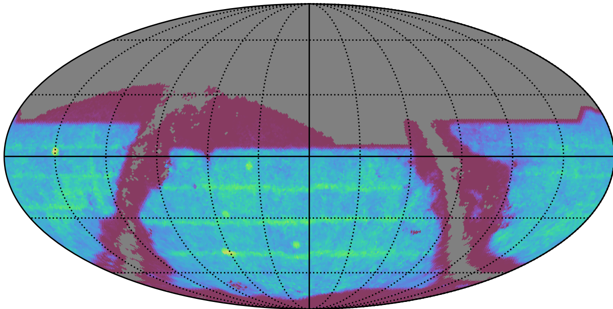
weather_cloudso4v3.4_10yrs : SNSLMetric
