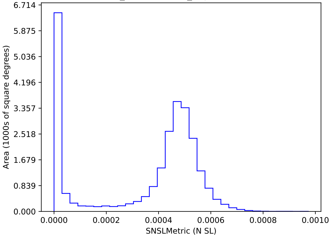
weather_cloudso4v3.4_10yrs : SNSLMetric
