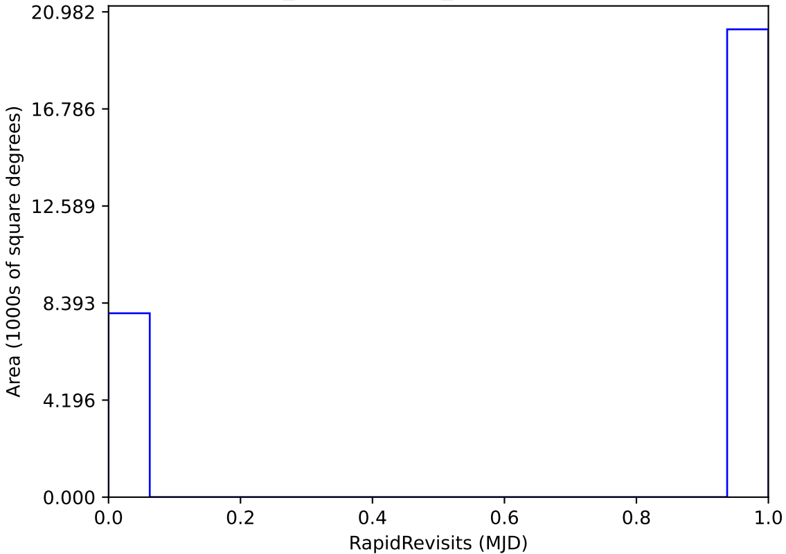
weather_cloudso4v3.4_10yrs : RapidRevisits
