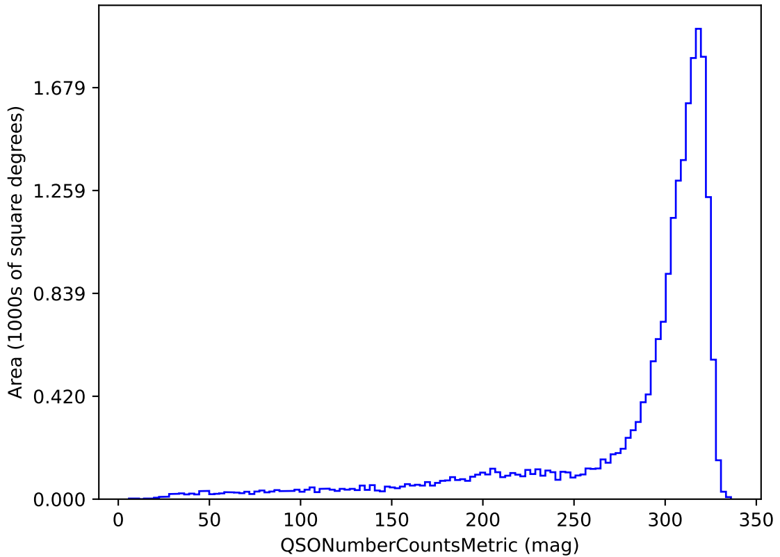
weather_cloudso4v3.4_10yrs u band and non-DD: QSONumberCountsMetric
