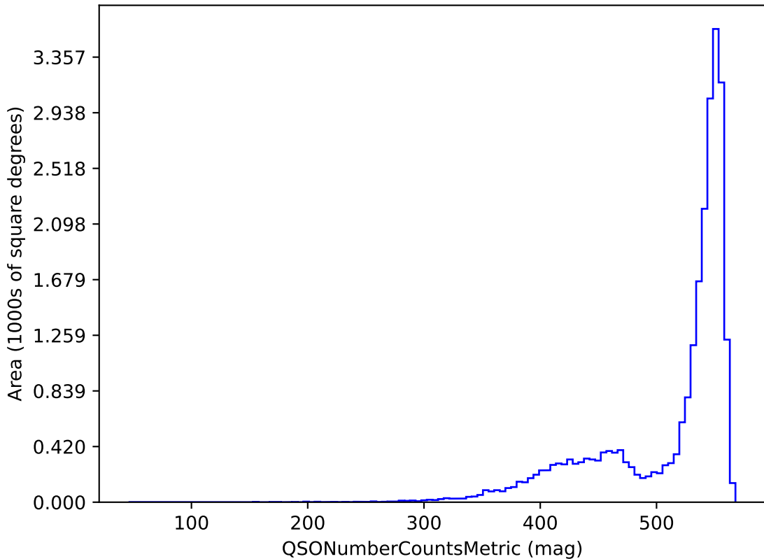
weather_cloudso4v3.4_10yrs i band and non-DD: QSONumberCountsMetric
