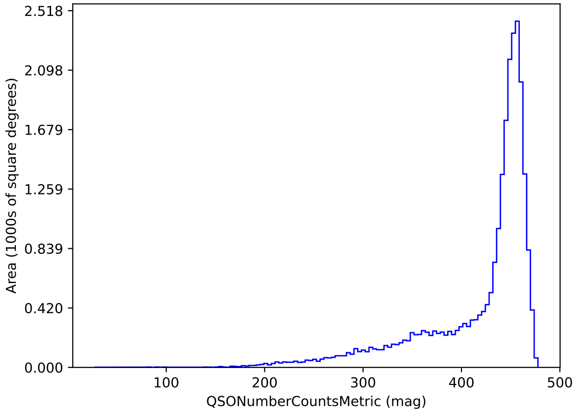
weather_cloudso4v3.4_10yrs g band and non-DD: QSONumberCountsMetric
