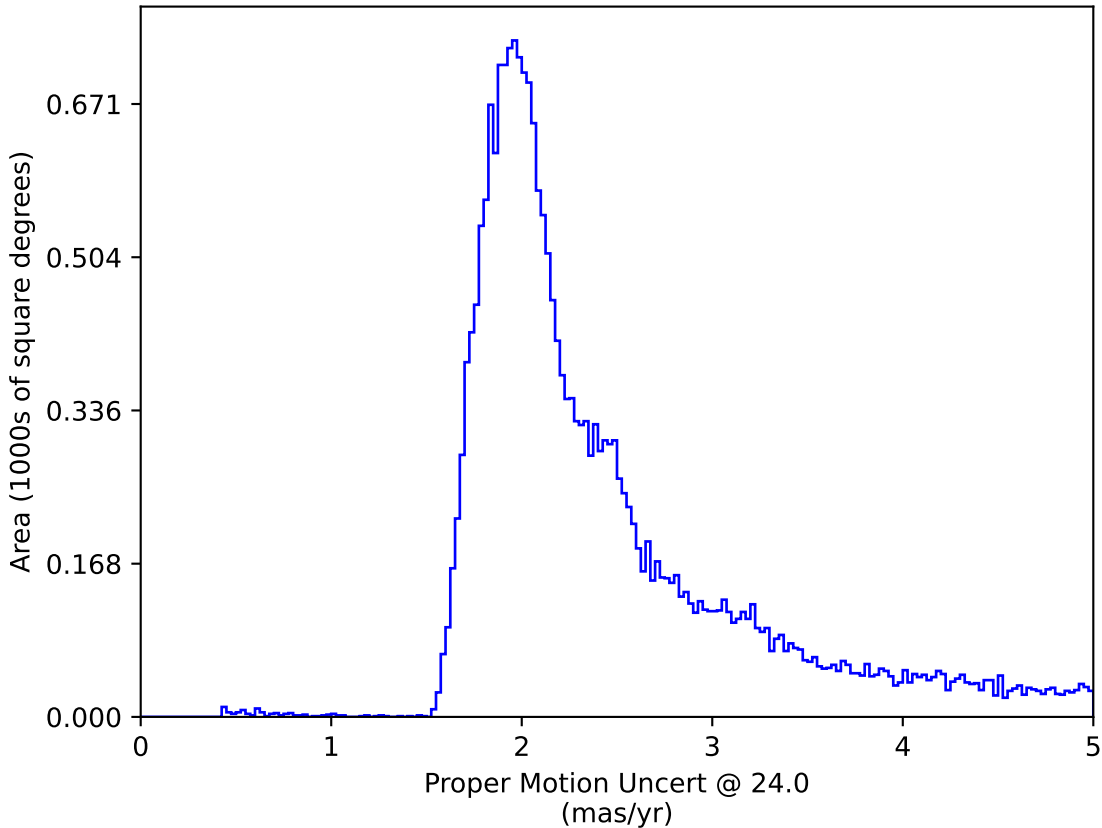
weather_cloudso4v3.4_10yrs : Proper Motion Uncert @ 24.0
