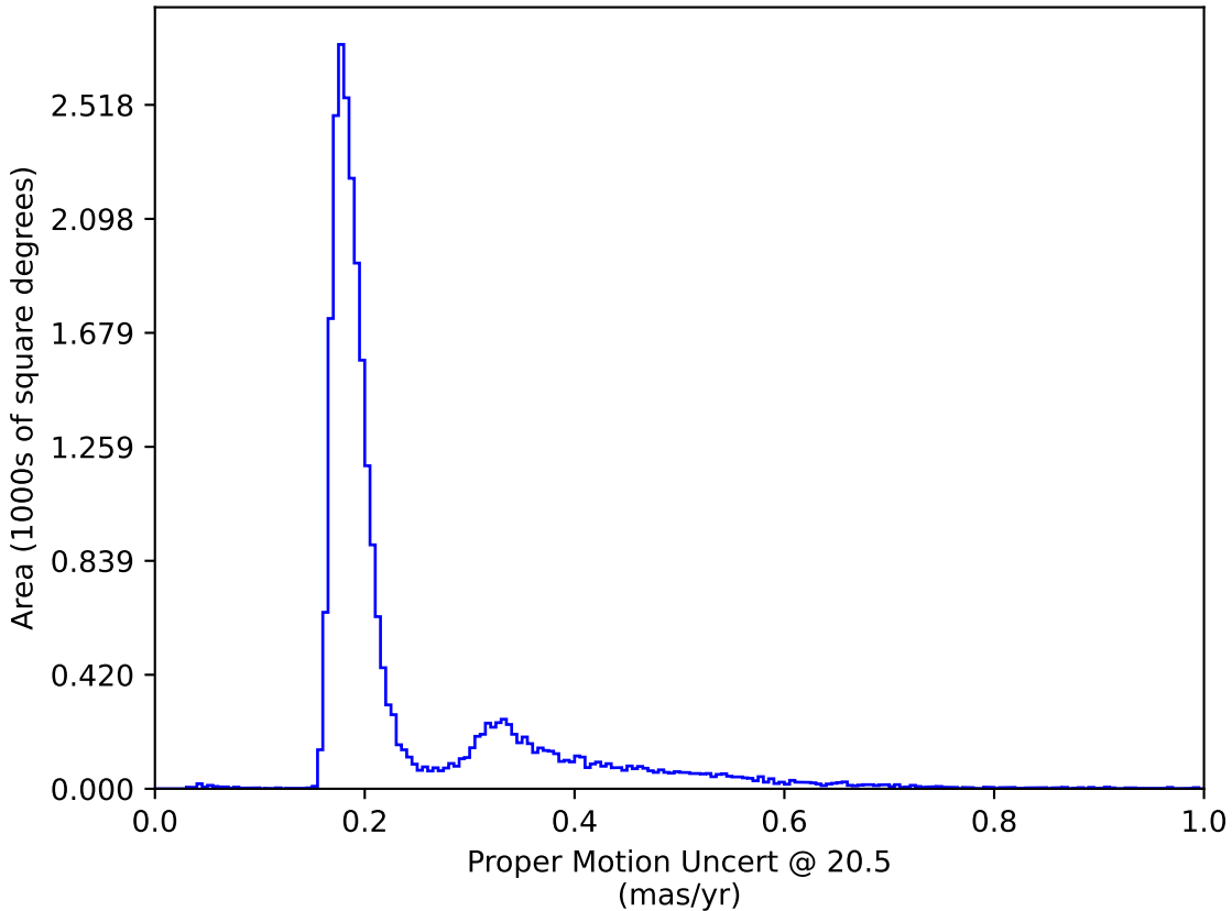
weather_cloudso4v3.4_10yrs : Proper Motion Uncert @ 20.5
