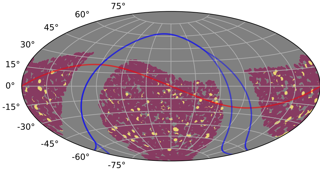
weather_cloudso4v3.4_10yrs : PrestoKNe_score_s
