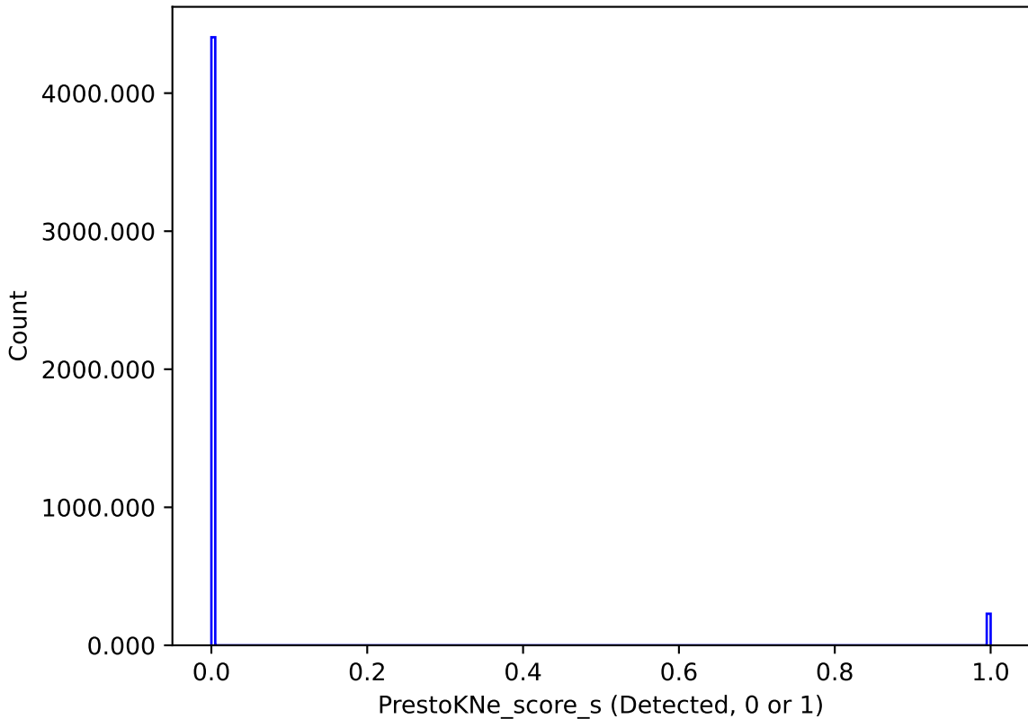
weather_cloudso4v3.4_10yrs : PrestoKNe_score_s
