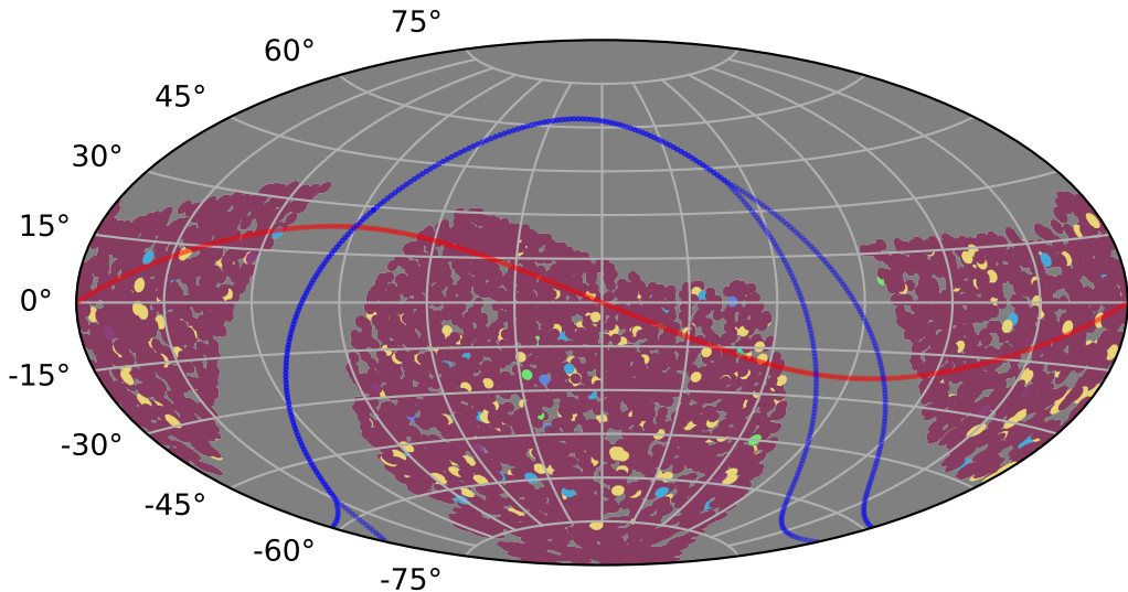
weather_cloudso4v3.4_10yrs : PrestoKNe_score_p
