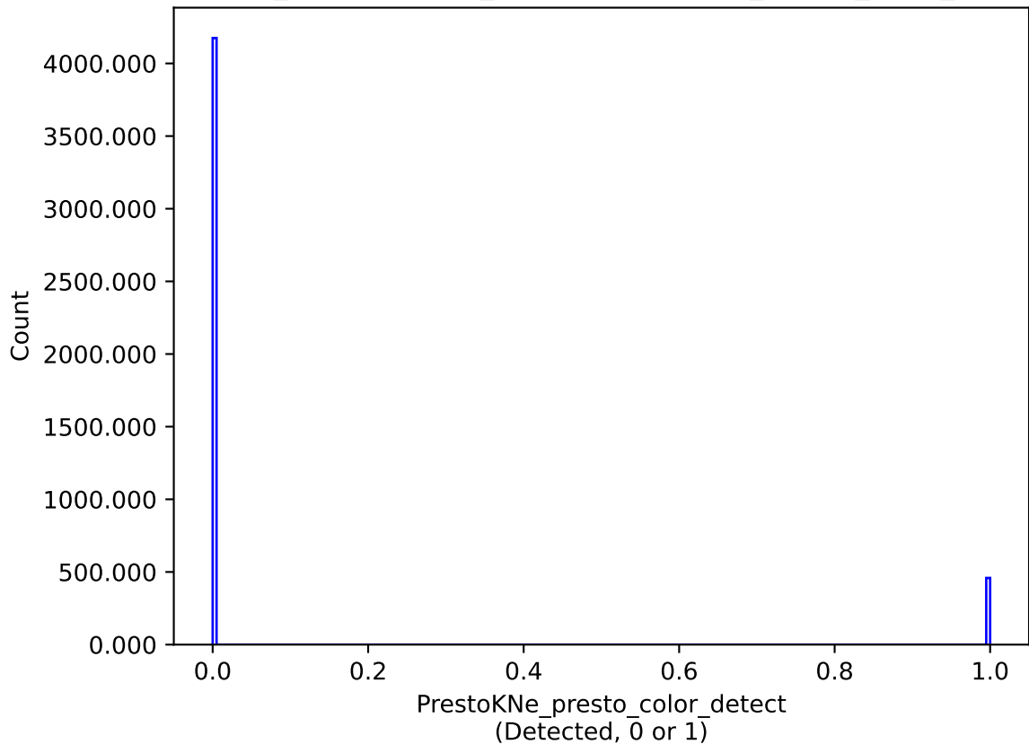
weather_cloudso4v3.4_10yrs : PrestoKNe_presto_color_detect
