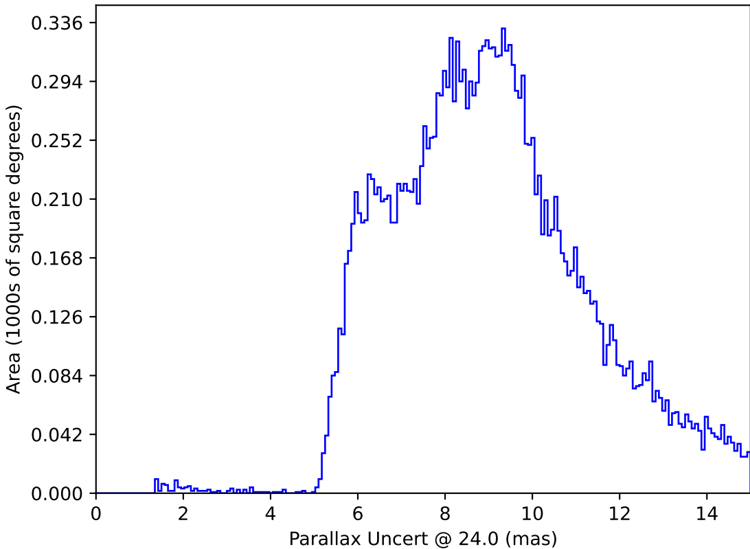
weather_cloudso4v3.4_10yrs : Parallax Uncert @ 24.0
