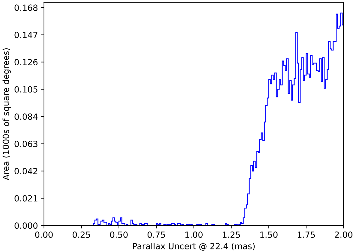
weather_cloudso4v3.4_10yrs : Parallax Uncert @ 22.4
