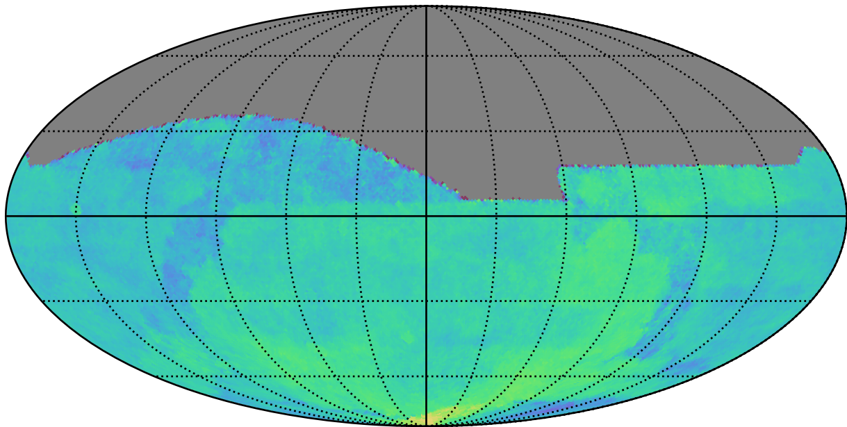
weather_cloudso4v3.4_10yrs : Parallax Coverage @ 24.0
