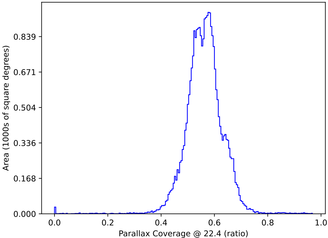
weather_cloudso4v3.4_10yrs : Parallax Coverage @ 22.4
