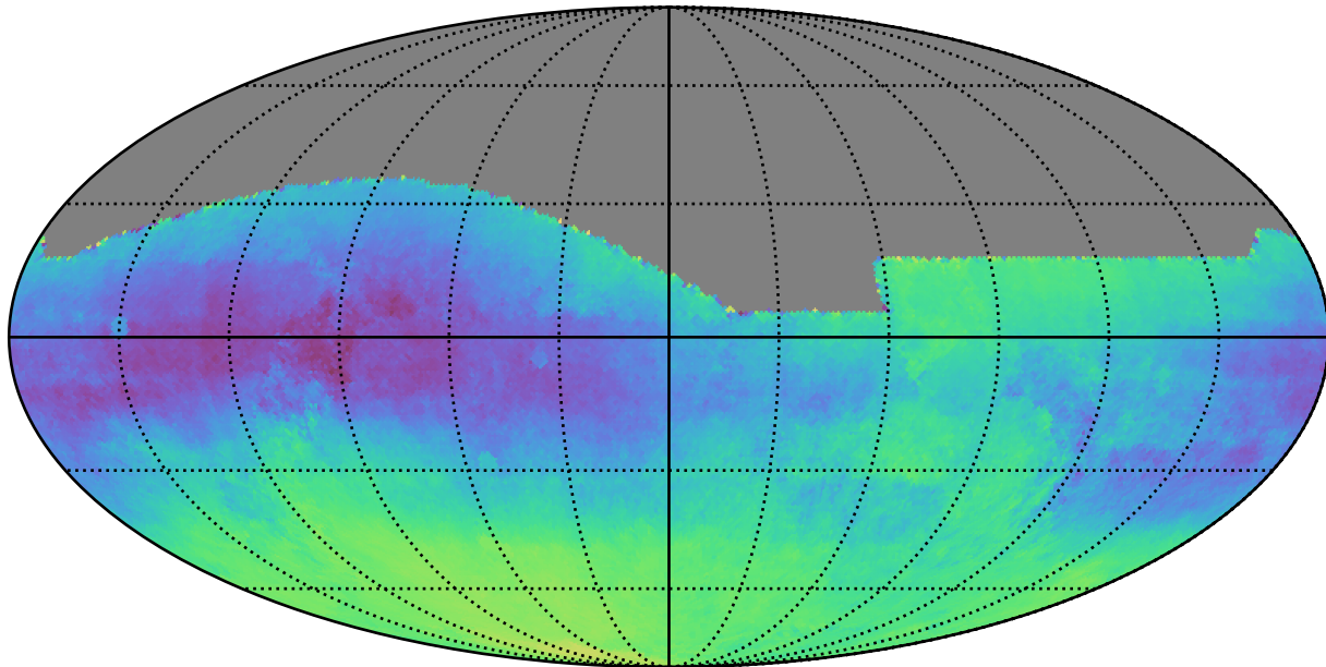
weather_cloudso4v3.4_10yrs : Parallax-DCR degeneracy @ 24.0
