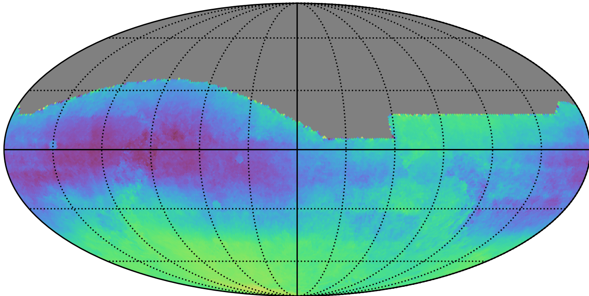
weather_cloudso4v3.4_10yrs : Parallax-DCR degeneracy @ 22.4
