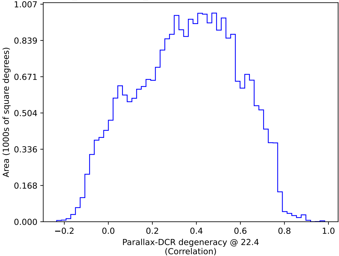
weather_cloudso4v3.4_10yrs : Parallax-DCR degeneracy @ 22.4
