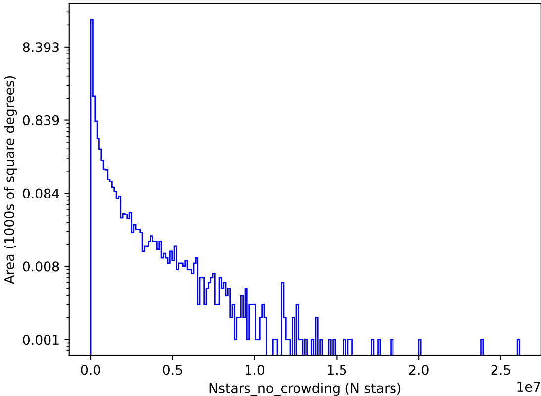
weather_cloudso4v3.4_10yrs y: Nstars_no_crowding
