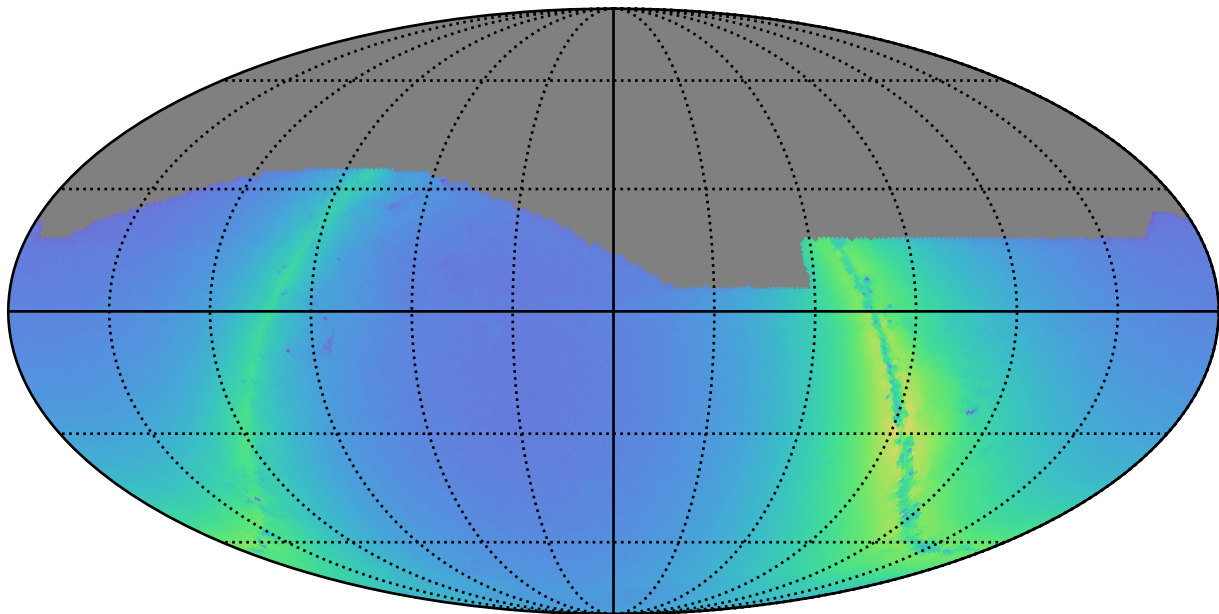
weather_cloudso4v3.4_10yrs r: Nstars_no_crowding
