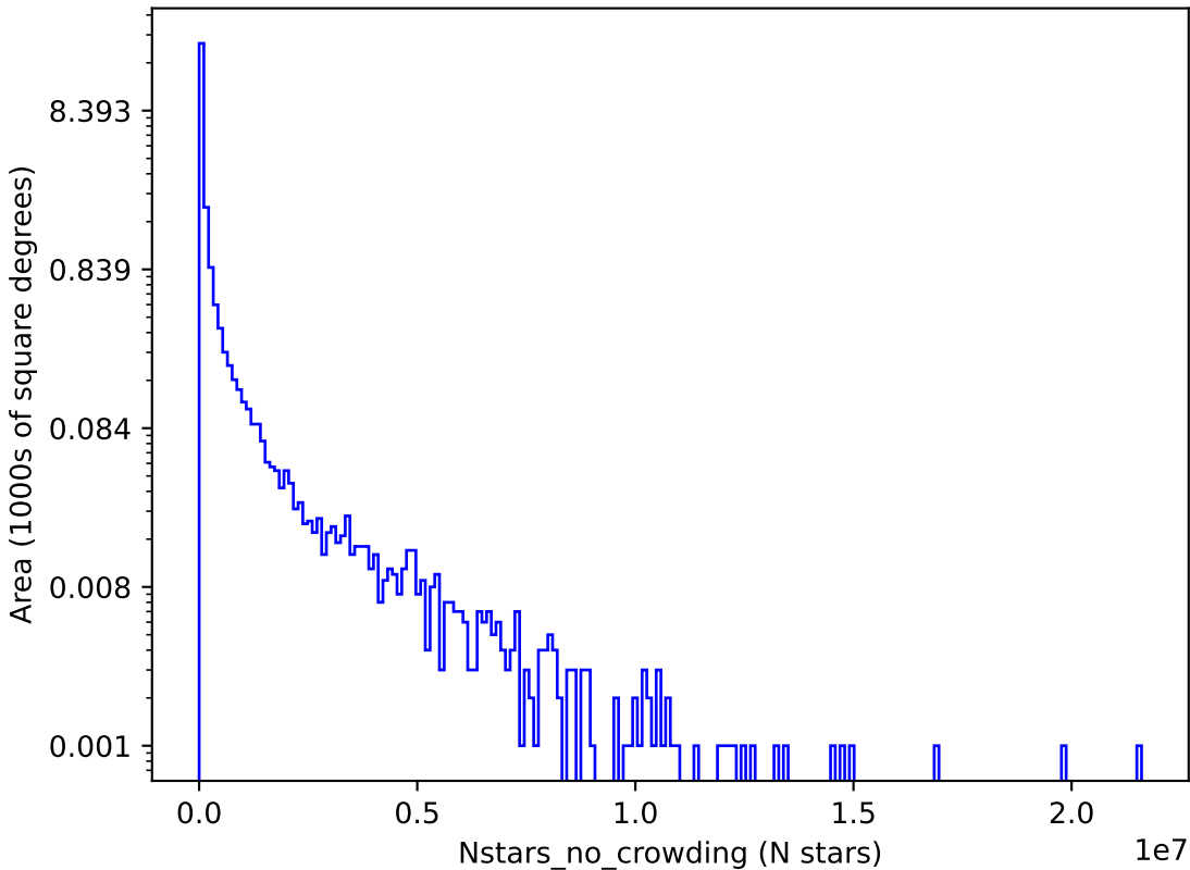
weather_cloudso4v3.4_10yrs r: Nstars_no_crowding
