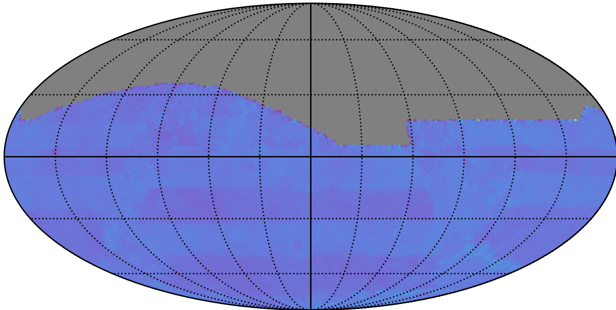
weather_cloudso4v3.4_10yrs : Normalized Proper Motion Uncert @ 24.0
