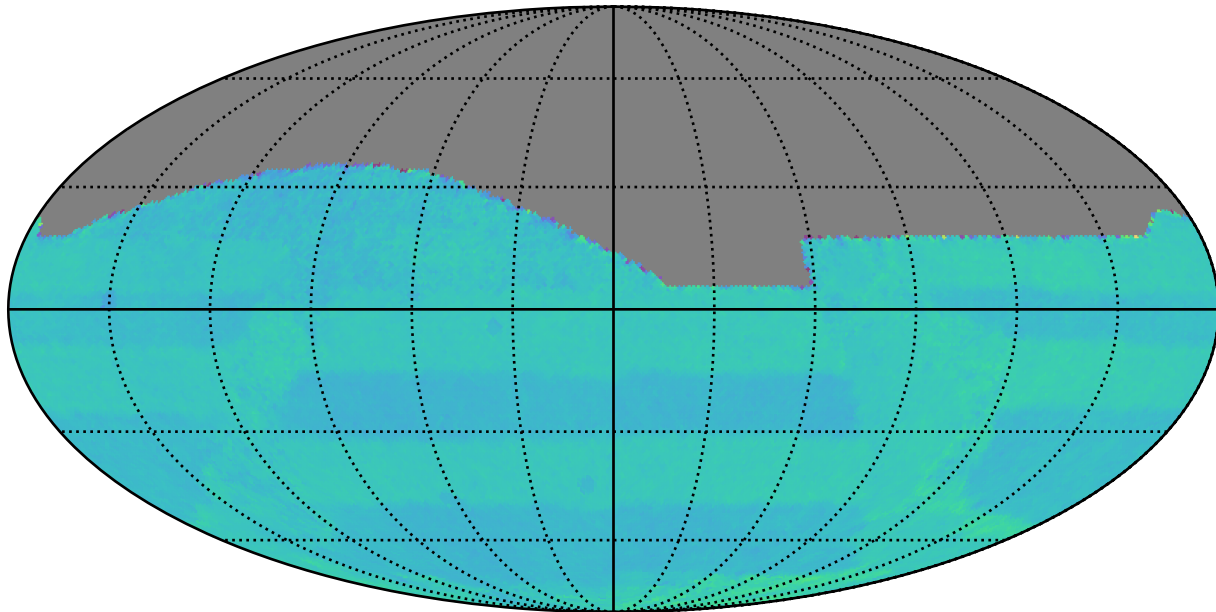
weather_cloudso4v3.4_10yrs : Normalized Proper Motion Uncert @ 20.5
