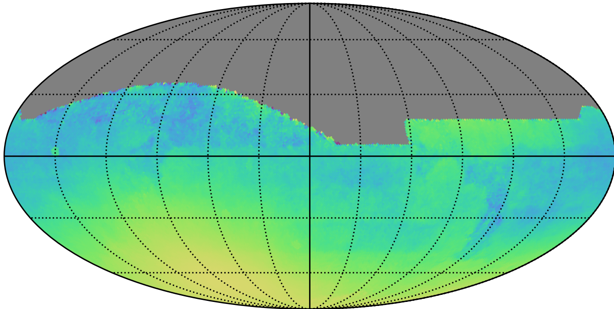
weather_cloudso4v3.4_10yrs : Normalized Parallax Uncert @ 24.0
