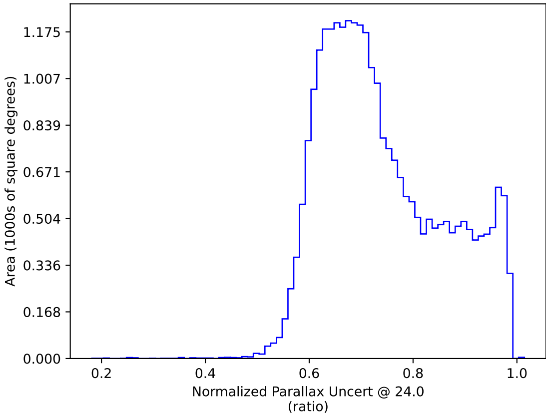
weather_cloudso4v3.4_10yrs : Normalized Parallax Uncert @ 24.0
