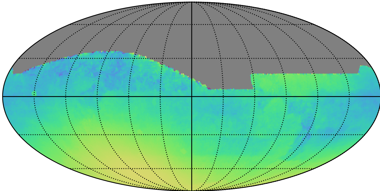
weather_cloudso4v3.4_10yrs : Normalized Parallax Uncert @ 22.4
