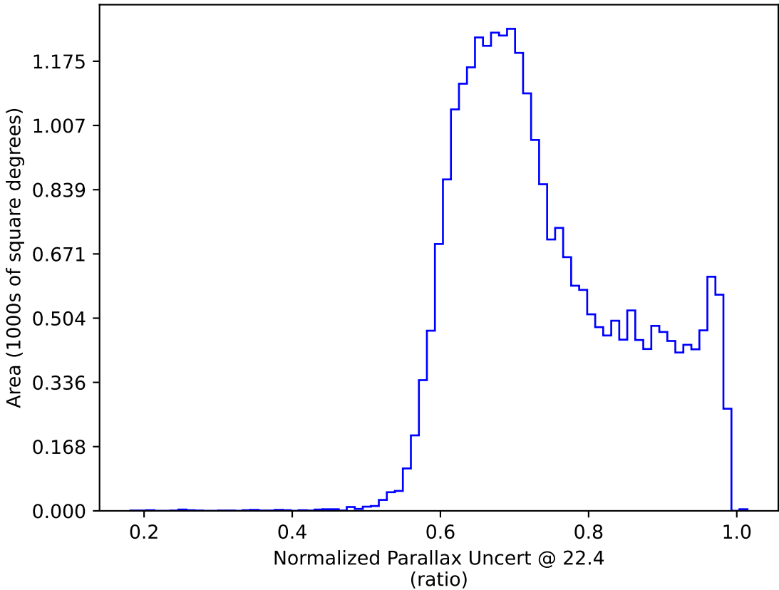
weather_cloudso4v3.4_10yrs : Normalized Parallax Uncert @ 22.4
