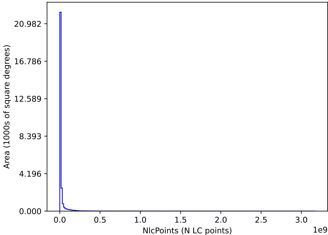
weather_cloudso4v3.4_10yrs : NlcPoints
