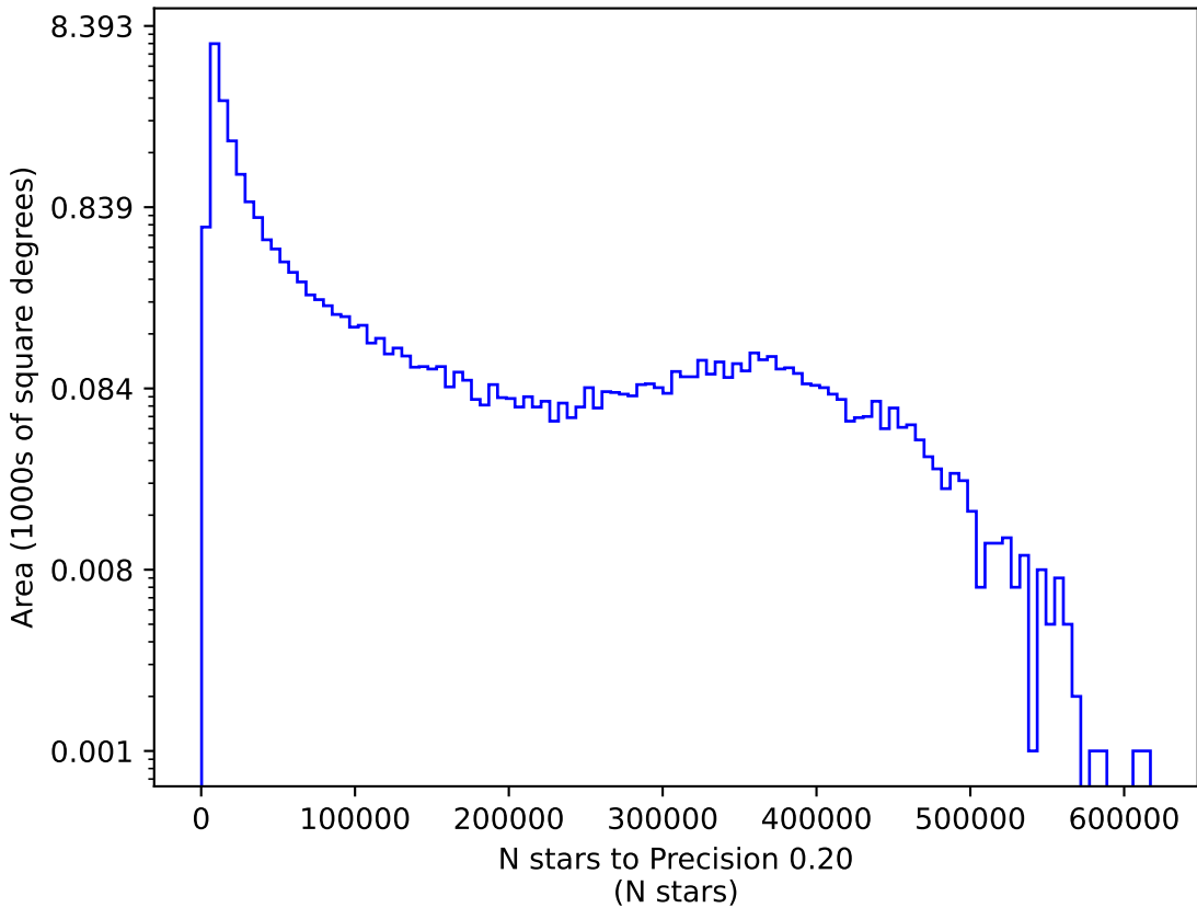
weather_cloudso4v3.4_10yrs y: N stars to Precision 0.20
