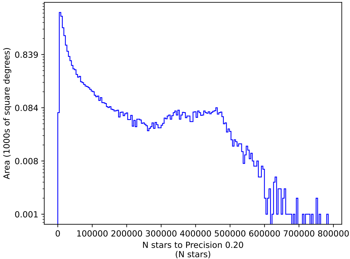
weather_cloudso4v3.4_10yrs r: N stars to Precision 0.20
