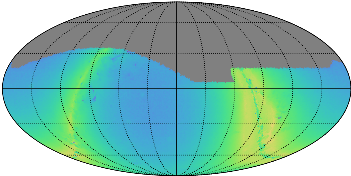
weather_cloudso4v3.4_10yrs g: N stars to Precision 0.20
