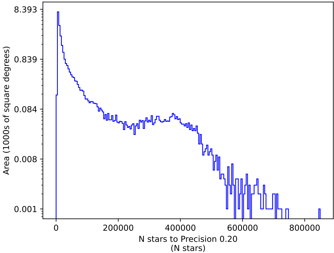
weather_cloudso4v3.4_10yrs g: N stars to Precision 0.20
