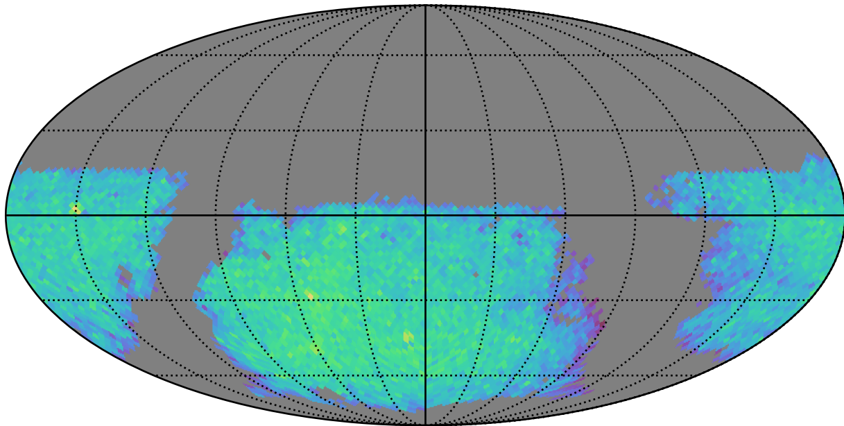
weather_cloudso4v3.4_10yrs gi: LVDwarfs
