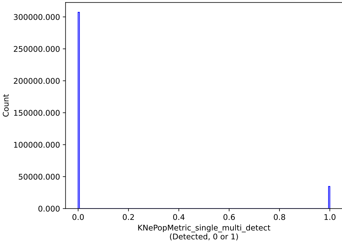
weather_cloudso4v3.4_10yrs single model: KNePopMetric_single_multi_detect
