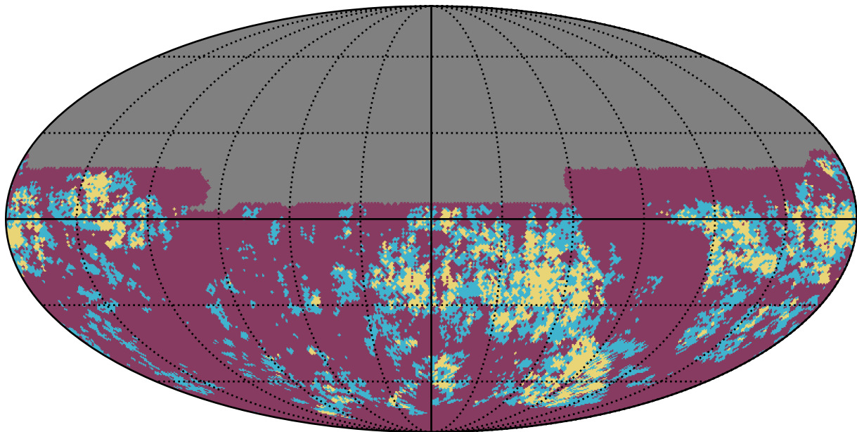
weather_cloudso4v3.4_10yrs y band: Gaps_7hr
