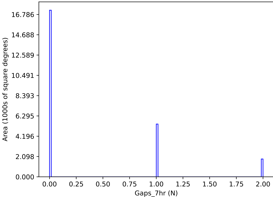
weather_cloudso4v3.4_10yrs y band: Gaps_7hr
