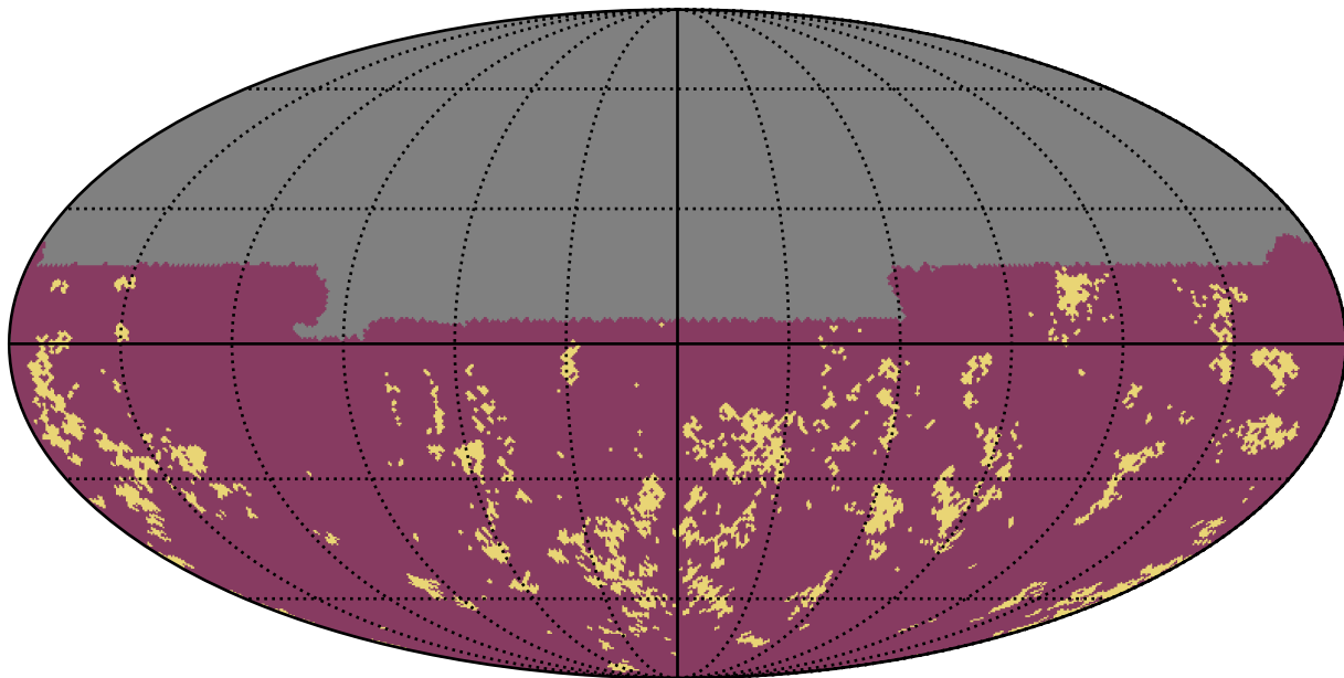
weather_cloudso4v3.4_10yrs u band: Gaps_7hr
