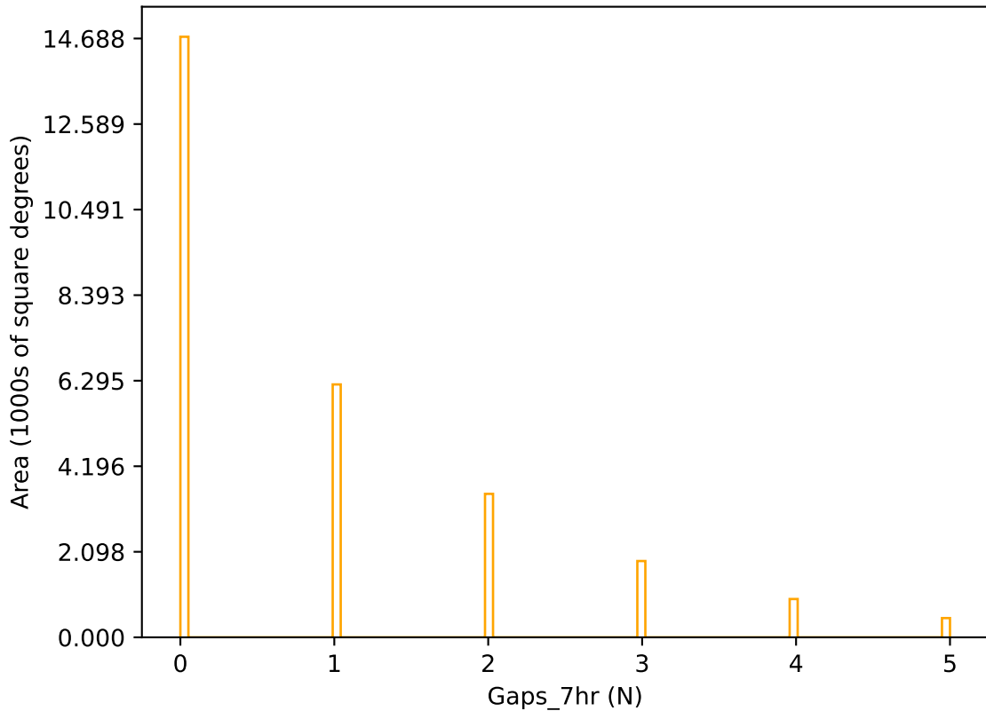
weather_cloudso4v3.4_10yrs r band: Gaps_7hr
