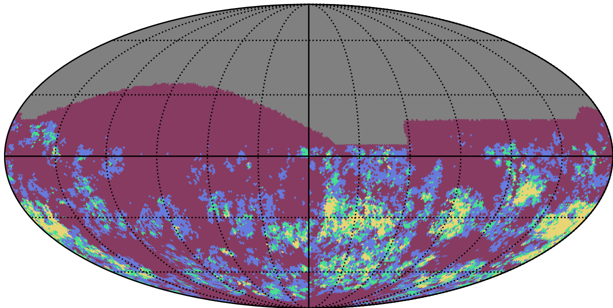
weather_cloudso4v3.4_10yrs i band: Gaps_7hr
