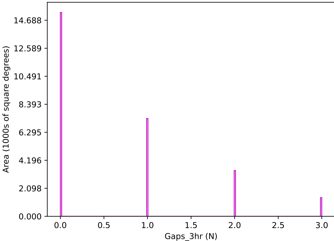
weather_cloudso4v3.4_10yrs z band: Gaps_3hr
