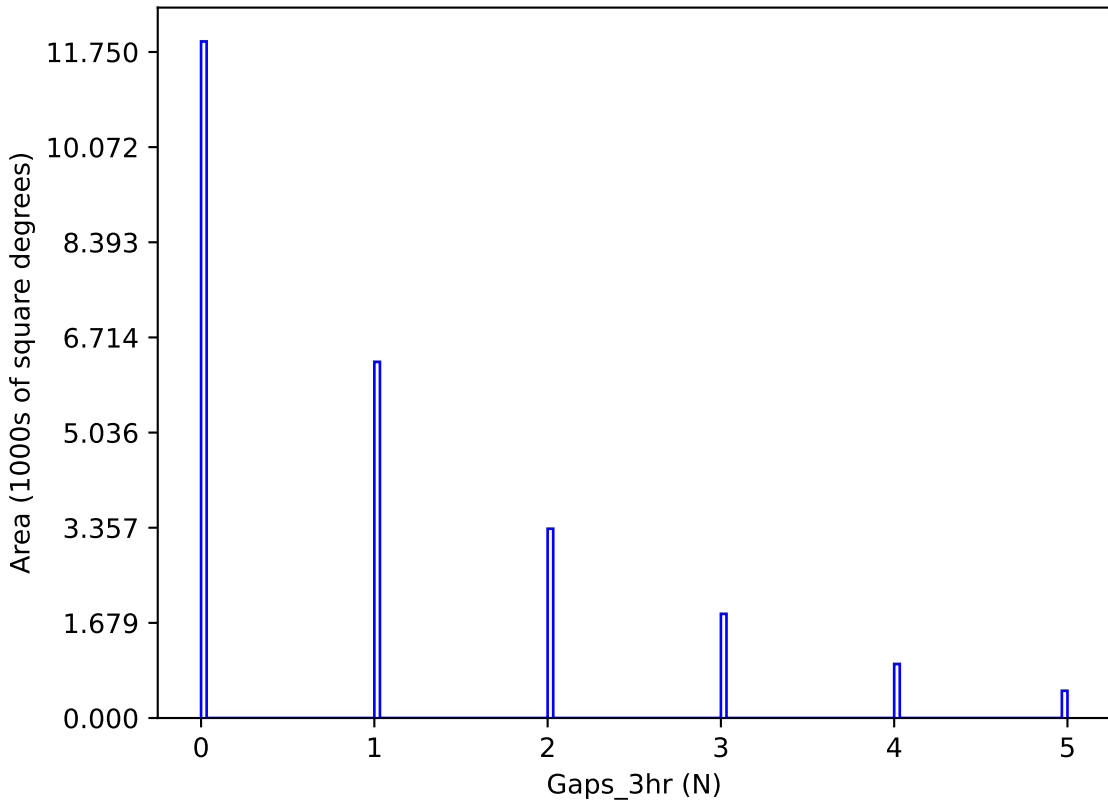
weather_cloudso4v3.4_10yrs y band: Gaps_3hr
