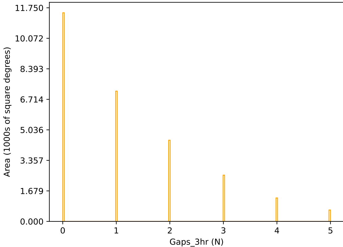
weather_cloudso4v3.4_10yrs r band: Gaps_3hr
