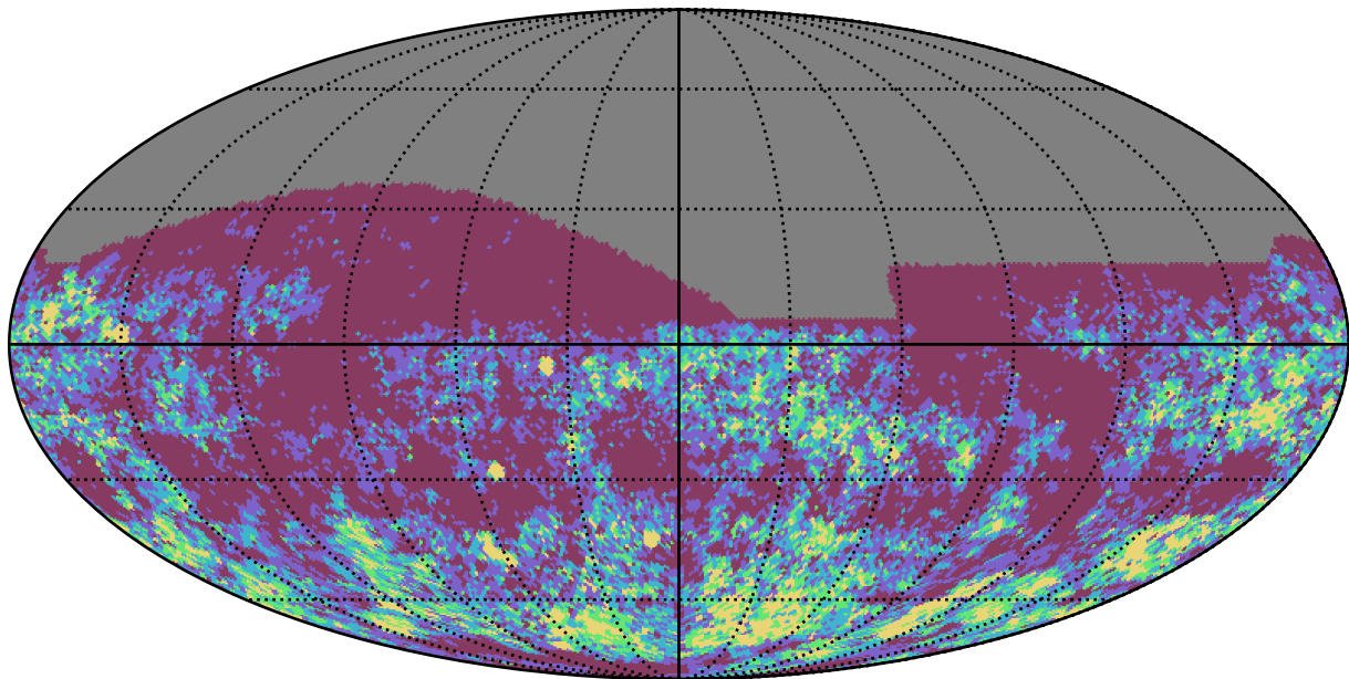
weather_cloudso4v3.4_10yrs i band: Gaps_3hr
