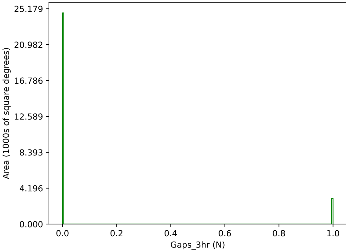
weather_cloudso4v3.4_10yrs g band: Gaps_3hr
