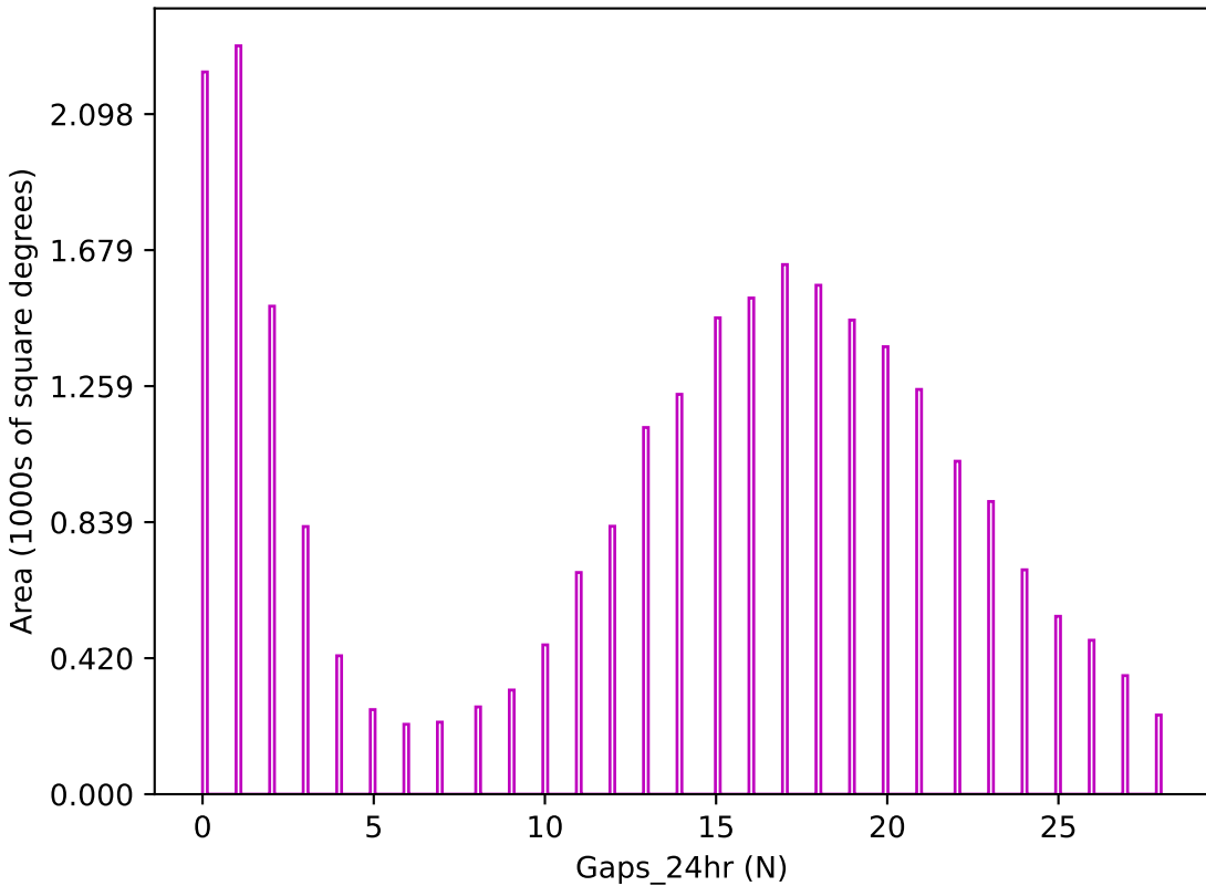
weather_cloudso4v3.4_10yrs z band: Gaps_24hr
