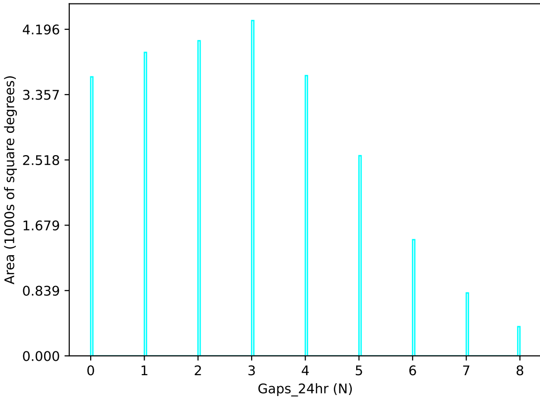
weather_cloudso4v3.4_10yrs u band: Gaps_24hr
