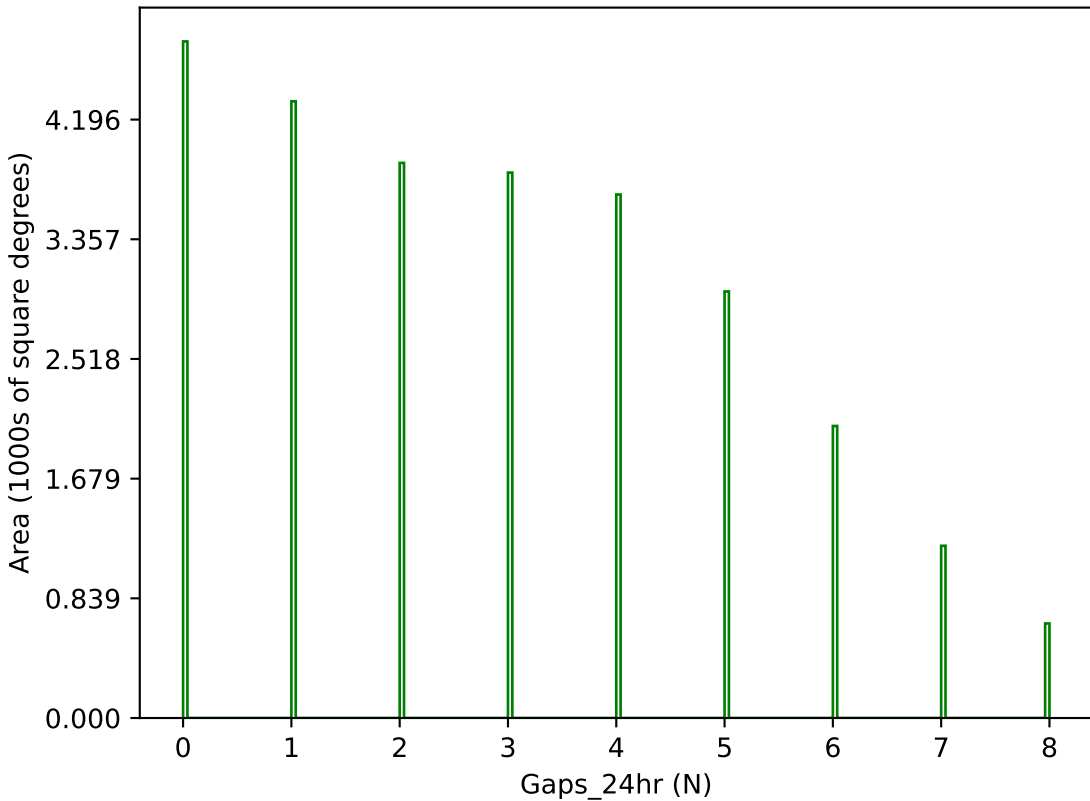
weather_cloudso4v3.4_10yrs g band: Gaps_24hr
