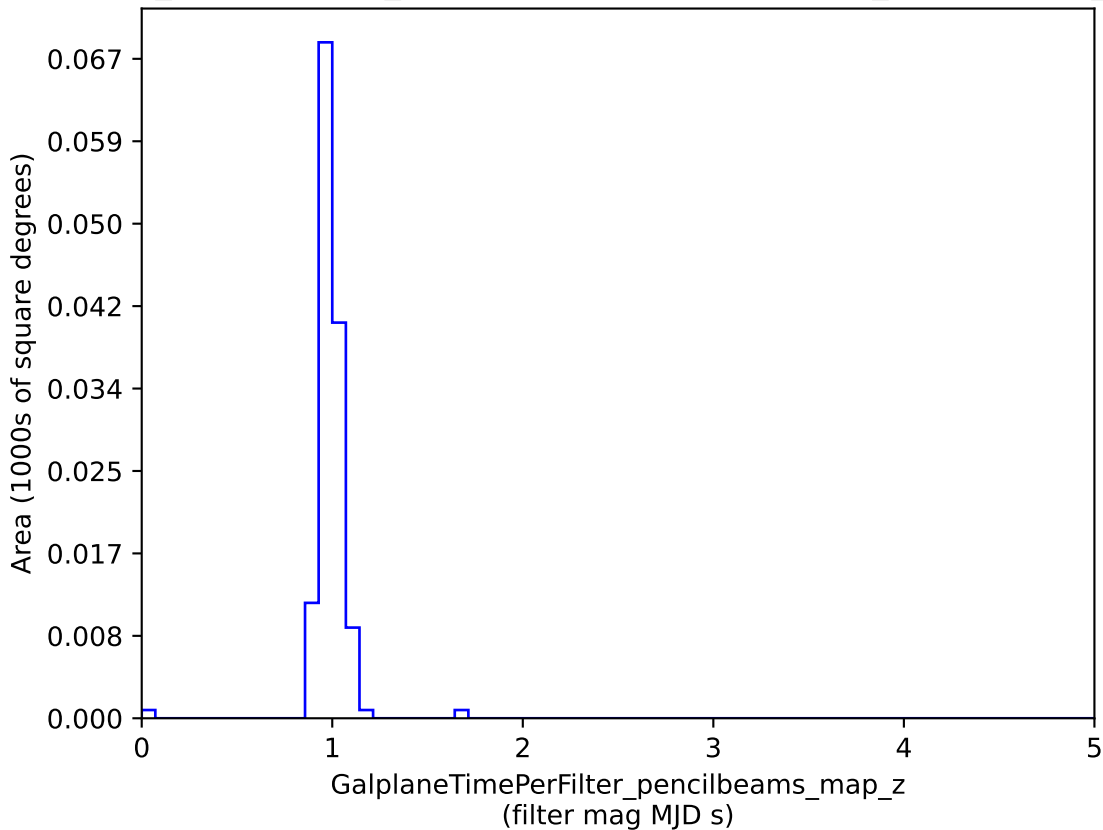
weather_cloudso4v3.4_10yrs : GalplaneTimePerFilter_pencilbeams_map_z
