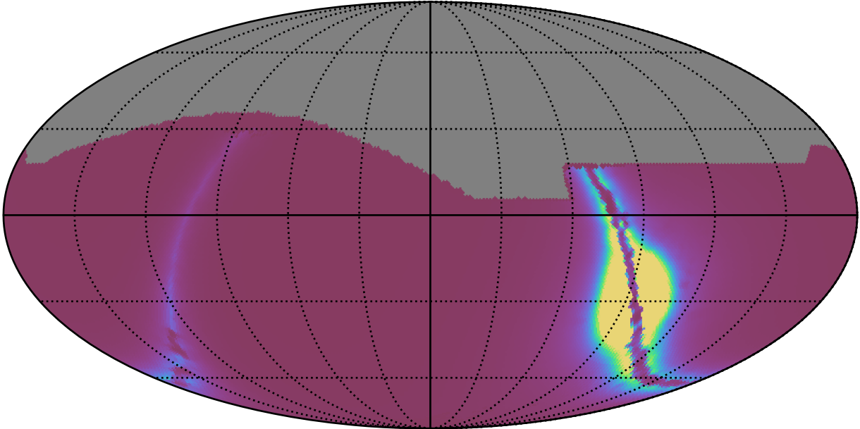
weather_cloudso4v3.4_10yrs : GalplaneFootprintMetric_xray_binaries_map_Tau_73_0
